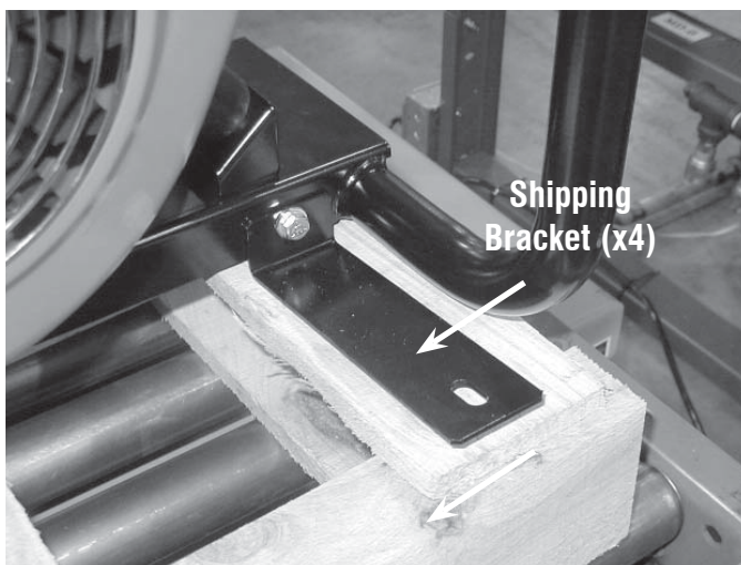
Figure 1 - Bracket Removal
